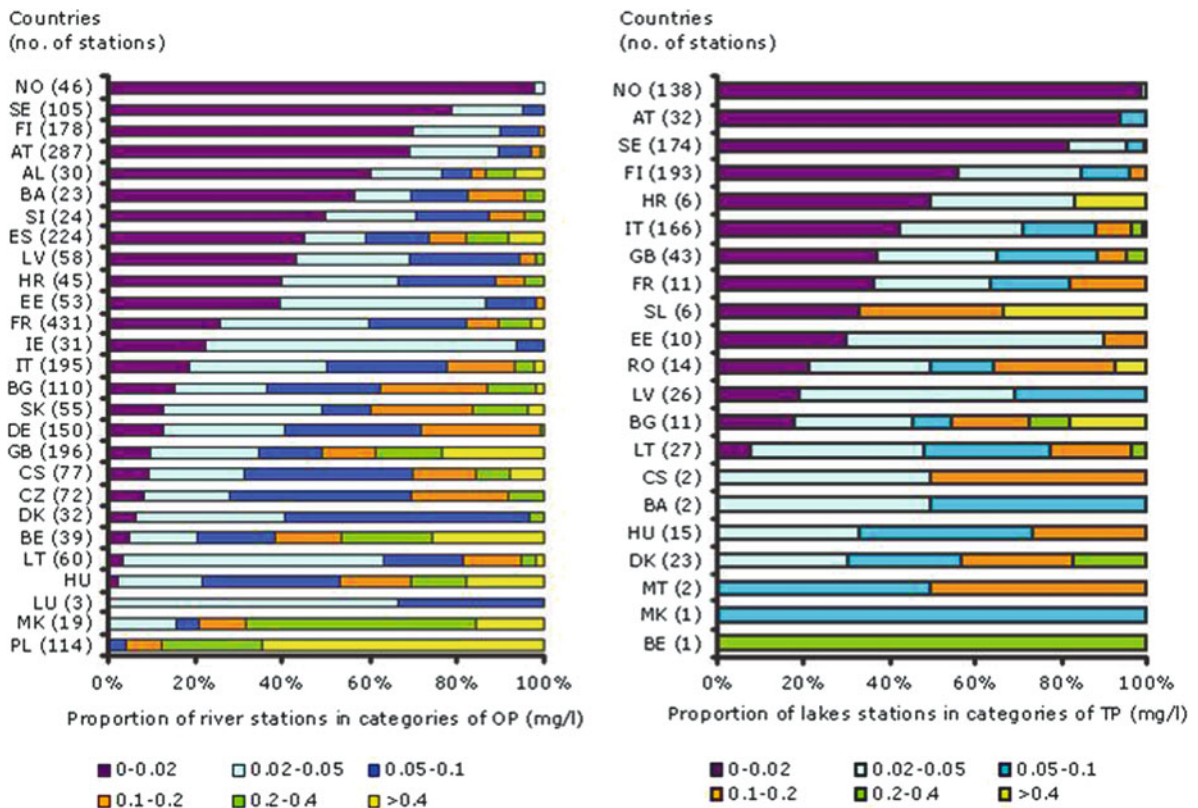
Fig. 1.3 Concentration of phosphorus in rivers (left; soluble reactive phosphate) and lakes (right; total phosphorus) in European countries. The number of monitoring stations in each country is given in brackets. Figures are based on the most recent
