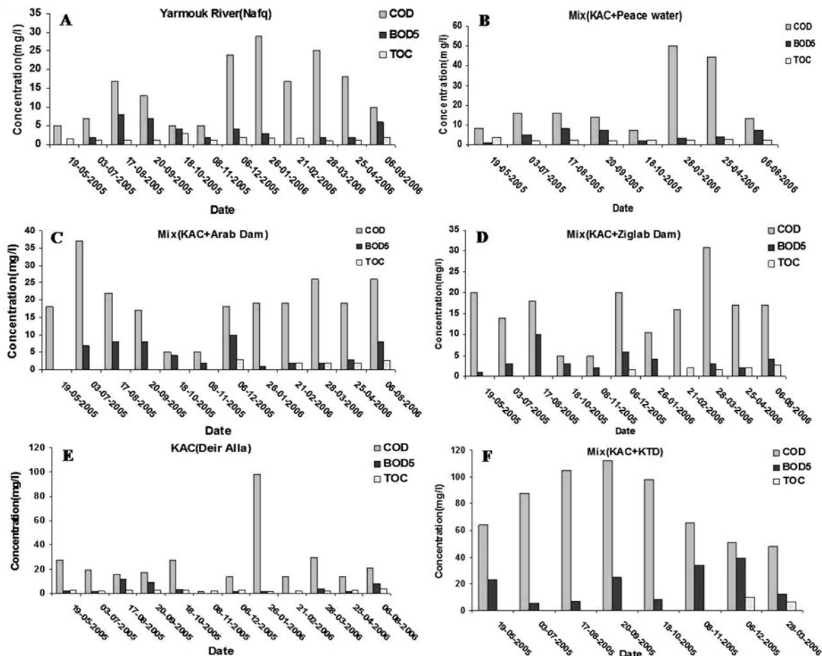
Fig. 3.9 Concentrations of COD, BOD 5 , and TOC in the sampled locations of the study area. (a) Yarmouk River; (b) mixture of KAC and Peace Water; (c) mixture of KAC and Arab Dam
